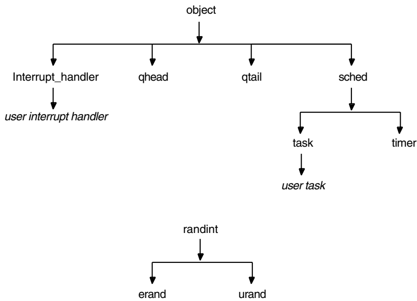
Figure 10–1 Inheritance Diagram for the task Package
